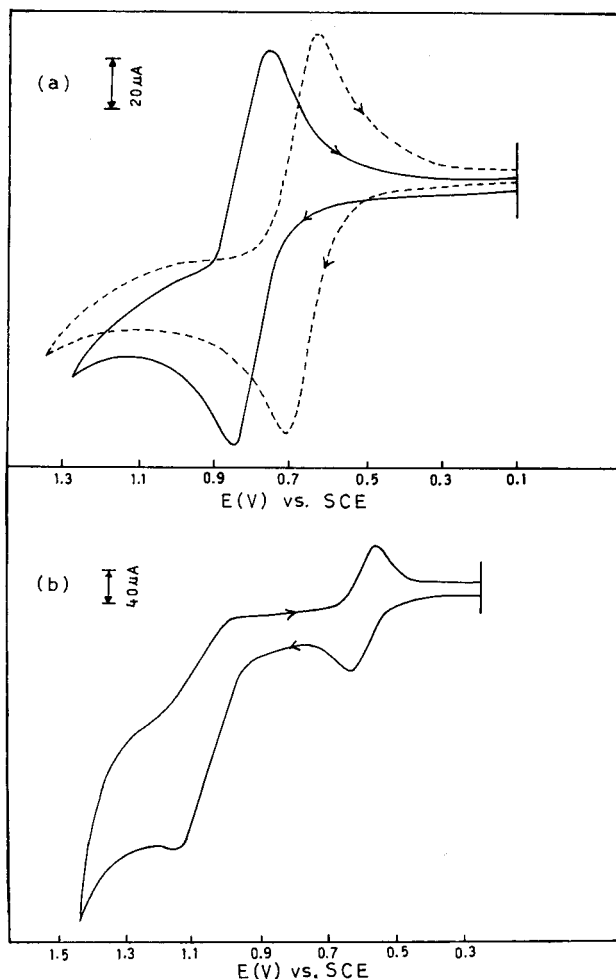
Figure 3. 3. Cyclic voltammograms in acetonitrile (0.1 M TBAP) at a platinum working electrode. The solute concentration and scan rate are \sim 10^{-3} M and 50 mV S -1 , respectively: (a) trans – cis – cis (5d) (—) cis – trans – cis (7d) (---); (b) trans – cis – cis (6b).
