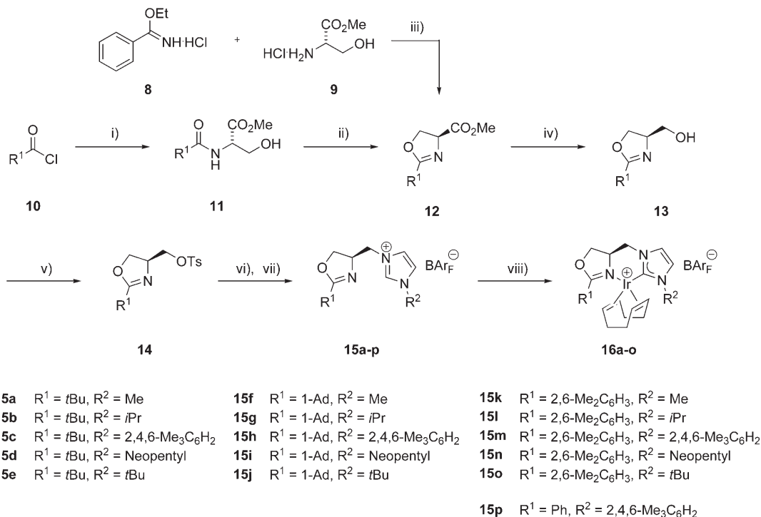
Scheme 2. Synthesis of iridium complexes F : i) ( S )-serine methyl ester hydrochloride, NEt 3 , CH 2 Cl 2 , RT, 10 h, (80–93 %); ii) Burgess reagent, THF, reflux, 4 h, (65–72 %); iii) 1,2-dichloroethane, reflux, 20 h, (91 %); iv) DIBAL, THF, RT, 12 h, (52–78 %); v) NEt 3 , TsCl, CH 2 Cl 2 , RT, (50–83 %); vi) imidazole, DMF, 80 °C, 8 h; vii) NaBAR F (BAR F − = tetrakis[3,5-bis(trifluoromethyl)phenyl]borate), acetone, RT, 15 min, (50–78 % over two steps); viii) [(η 4 -cod)IrCl] 2 , NaOtBu, THF, 3 h, (48–83 %).
