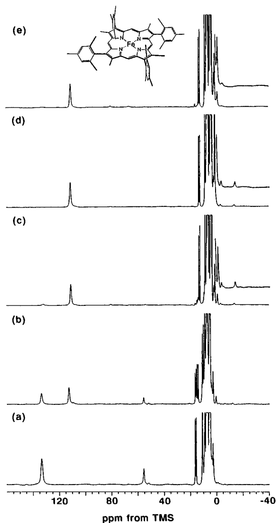
Figure 1. ^1\text{H} -NMR spectra for the titration of (\text{P}^*)\text{Fe}^{\text{IV}}\text{O}(\text{ClO}_4) with imidazole at -80^\circ\text{C} in dichloromethane- d_2 . Concentration of iron porphyrin: 5.3 mM. Imidazole added: (a) 0.0 equiv; (b) 0.5 equiv; (c) 1.0 equiv; (d) meso- d_4 (\text{P}^*)\text{Fe}^{\text{IV}}\text{O}(\text{ClO}_4) with 1.0 equiv of imidazole; (e) (\text{P}^*)\text{Fe}^{\text{IV}}\text{O}(\text{ClO}_4) with 1.0 equiv of imidazole- d_3 .
