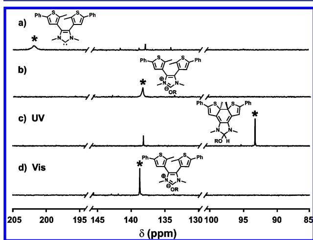
Figure 5. Quantitative 13 C NMR spectra collected sequentially in C 6 D 6 over the course of the following experiment: A sample of (a) 1o labeled at the C2 position with a 13 C atom (i.e., 1o *; [ 1o *] 0 = 1.0 × 10 −2 M) (b) was treated with equimolar quantities of 2-aminoethanol and ethyl acetate and (c) then exposed to UV irradiation for 1 h ( \lambda_{\text{irr}} = 313 nm; [ 1o *] 0 = 2.5 × 10 −3 M) and finally (d) irradiated with visible light for an additional 2 h ( \lambda_{\text{irr}} > 500 nm, [ 1o *] 0 = 1.0 × 10 −2 M). See text for additional details.
