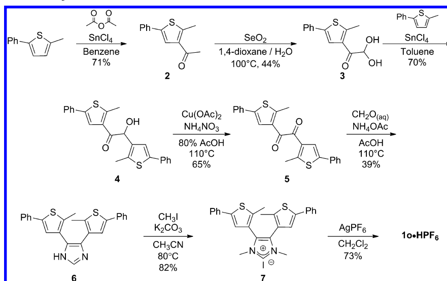
Scheme 2. Synthesis of 1o •HPF 6
