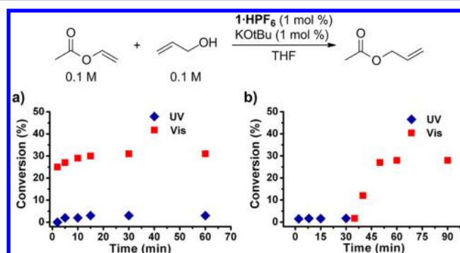
Figure 3. Plots of the percent of starting materials which have converted to products versus time for the condensation of vinyl acetate and allyl alcohol catalyzed by 1 (prepared in situ from 1o •HPF 6 and KOtBu) in THF. The reactions were monitored over time by GC using n -octane as an internal standard. (a) Two reactions were run concurrently with one vessel exposed to UV irradiation ( \lambda_{\text{irr}} = 313 nm) for 1 h prior to substrate addition (blue diamonds) and one kept under ambient light (red squares). (b) A single reaction vessel was exposed to UV irradiation ( \lambda_{\text{irr}} = 313 nm) for 1 h prior to substrate addition. The contents of the vessel were then stirred under UV light for 30 min (blue diamonds) prior to exposure to visible light ( \lambda_{\text{irr}} > 500 nm) (red squares).
