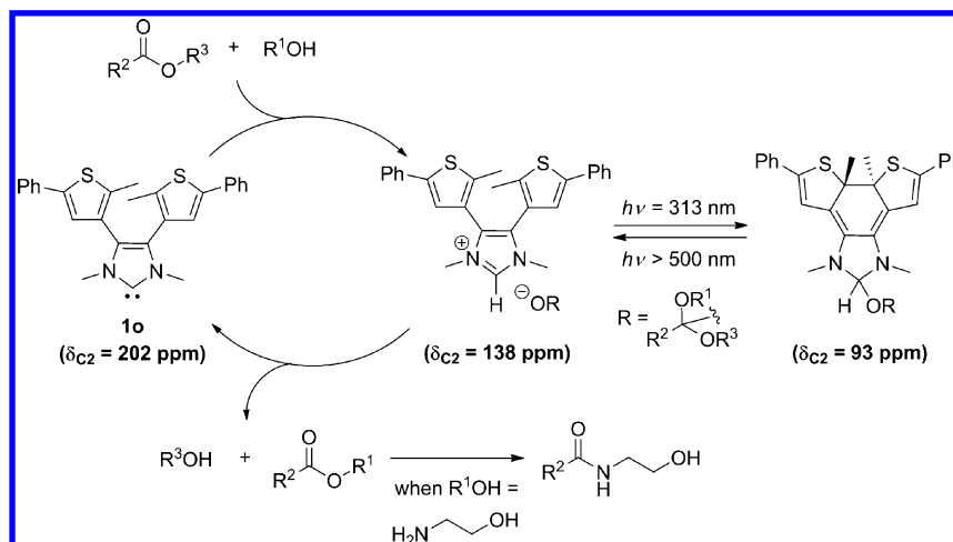
Scheme 3. Proposed Mechanism of Photoswitchable NHC Catalyzed Condensation Reactions
