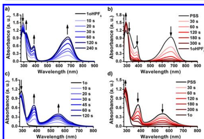
Figure 2. (a) UV–vis spectral changes of 1o •HPF 6 in C 6 H 6 upon UV irradiation ( \lambda_{\text{irr}} = 313 nm). (b) UV–vis spectrum in C 6 H 6 of 1o •HPF 6 at the photostationary state (PSS) reached after UV irradiation of 1o •HPF 6 for 240 s, and spectral changes of the PSS upon visible irradiation ( \lambda_{\text{irr}} > 500 nm). (c) UV–vis spectral changes of 1o (generated in situ by treatment of 1o •HPF 6 with 1.0 equiv of NaHMDS) in C 6 H 6 upon UV irradiation ( \lambda_{\text{irr}} = 313 nm). (d) UV–vis spectrum in C 6 H 6 of 1o , the photostationary state (PSS) reached after UV irradiation of 1o for 120 s, and spectral changes of the PSS upon visible irradiation ( \lambda_{\text{irr}} > 500 nm). In all cases, the initial concentration of 1o was 4 \times 10^{-5} M and the spectra were recorded after irradiation for the indicated amount of time. The arrows indicate the evolution of the spectral changes over time.
