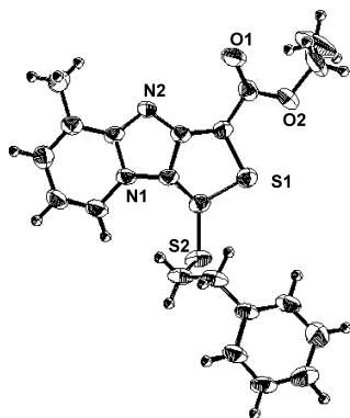
Fig. 2. ORTEP Drawing of Compound 12o
