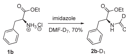
Scheme 4. N -Formylation of Phe-OEt·HCl ( 1b ) in DMF- D_7
