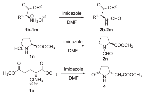
Scheme 2. N -Formylation of Amino Acids 1a – 1n and Formation of 4
