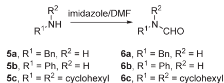
Scheme 3. N -Formylation of Amines 5a–5c
