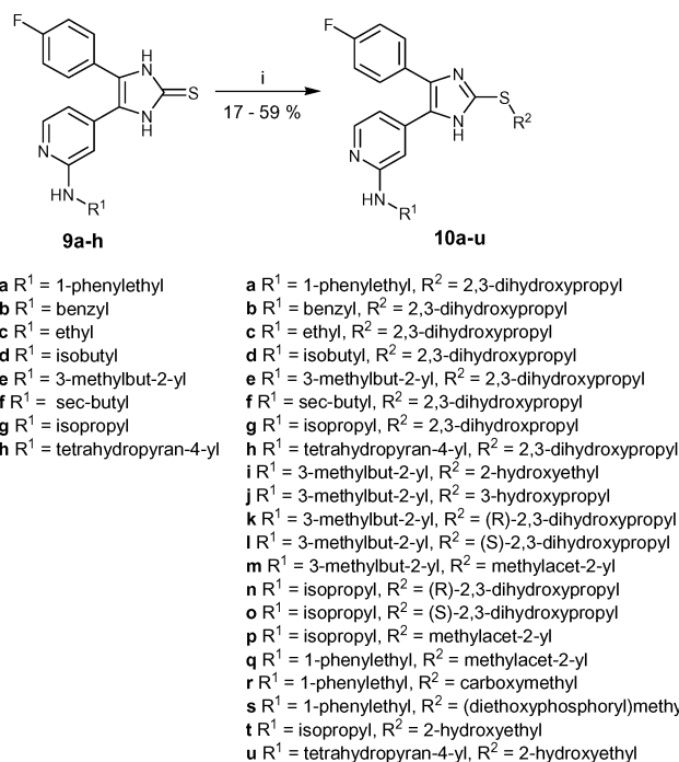
Scheme 4 Synthesis of the target compounds 10a–u ; reagents: (i) R 2 –X (X = Cl, Br, I), t -BuOK or EtONa, MeOH.
