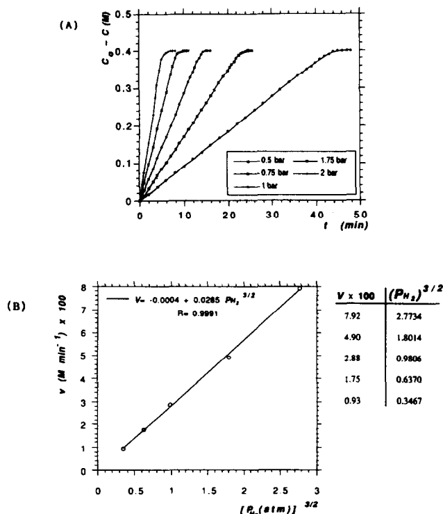
Fig. 4. Hydrogenation of 1-hexene catalysed by 2d ( T=62^\circ\text{C} ; [1-hexene] _0 = 0.4 M; [catalyst] = 3 \cdot 10^{-4} M). (A) Olefin concentration as a function of time for different hydrogen pressures. (B) Rate of hydrogenation as a function of hydrogen pressure.
