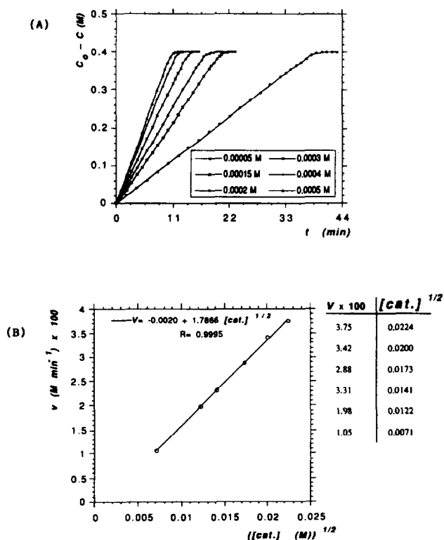
Fig. 3. Hydrogenation of 1-hexene catalysed by 2d ( P(\text{H}_2)=1 bar (0.987 atm); T=62^\circ\text{C} ; [1-hexene] _0 = 0.4 M). (A) Olefin concentration as a function of time for different catalyst concentrations. (B) Rate of hydrogenation as a function of catalyst concentration.
