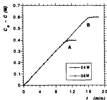
Fig. 2. Hydrogenation of 1-hexene catalysed by 2d ( P(\text{H}_2)=1 bar (0.987 atm); T=62^\circ\text{C} ; [catalyst] = 5 \cdot 10^{-4} M). Olefin concentration as a function of time: curve A, [\text{1-hexene}]_0 = 0.4 M; curve B, [\text{1-hexene}]_0 = 0.6 M.
