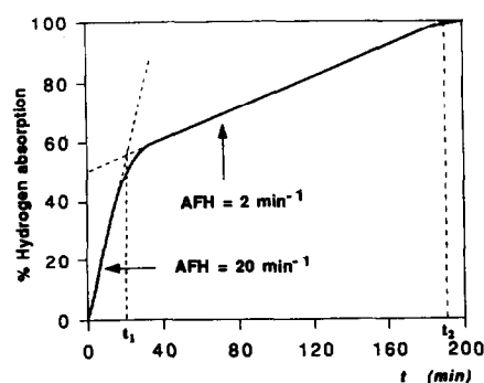
Fig. 1. AFH values for hydrogenation of 1,5-cyclooctadiene (0.4 M) by 2'a-Mg ( 10^{-3} \text{ M} ).
