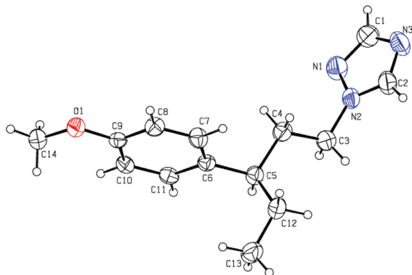
Figure 2. Molecular structure of compound 5d-R.
