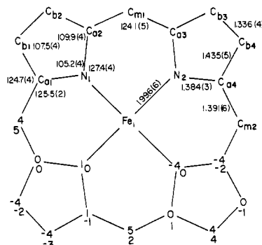
Figure 4. A formal diagram of a porphinato core displaying for Fe(THT) 2 (TPP) the averaged values of the unique chemical types of bond distances and bond angles. The numbers in parentheses are the estimated standard deviations calculated on the assumption that all values are drawn from the same population. On the lower half of the diagram the perpendicular displacements, in units of 0.01 Å, of each atom from the mean plane of the 24-atom core are shown. The upper value of each pair of values is that for molecule 1, the lower is that for molecule 2. The displacements of the centrosymmetrically related atoms are of the same magnitude and opposite sign.
