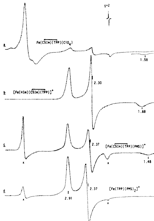
Figure 9. EPR spectra in methylene chloride/chloroform (10 K) for (a) \text{Fe}(\text{C}_5\text{Im})(\text{TPP})(\text{ClO}_4) showing both low-spin ( g = 2.86, 2.28, 1.58 ) and high-spin ( g = 5.90, 1.99 ) signals, (b) low-spin bis-N-ligated [\text{Fe}(\text{HIm})(\text{C}_5\text{Im})(\text{TPP})]^+ ( g = 2.90, 2.30, 1.68 ), (c) the EPR spectrum resulting from the addition of pentamethylene sulfide to \text{Fe}(\text{C}_5\text{Im})(\text{TPP})(\text{ClO}_4) ( g = 2.90, 2.37, 1.48 ) (bands marked (x) are due to a high-spin species (see text), and (d) [\text{Fe}(\text{TPP})(\text{PMS})_2]^+ ( g = 2.91, 2.37 ).
