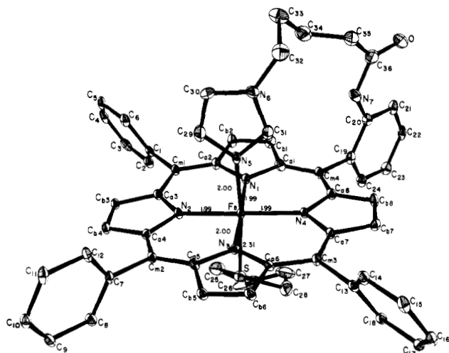
Figure 7. A computer-produced perspective view of the Fe(C5Im)-(TPP)(THT) molecule using 50% probability ellipsoids. The labels assigned to each atom are shown as are the distances around the iron(II) atom.
