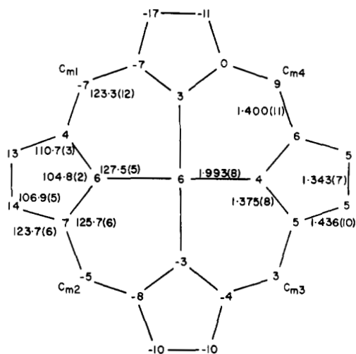
Figure 8. A formal diagram of the porphinato core of the Fe-(C5Im)(TPP)(THT) molecule. The core has the same relative orientation as that of Figure 7. Averaged bond parameters are shown along with the perpendicular displacements, in units of 0.01 Å, from the mean plane of the porphinato core.
