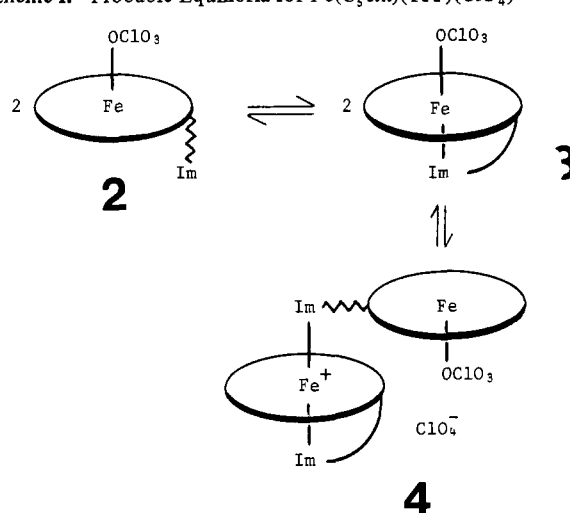
Scheme I. Probable Equilibria for \text{Fe}(\text{C}_5\text{Im})(\text{TPP})(\text{ClO}_4)
