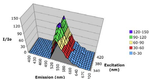
Figure 1. Fluorescence spectrum of DSEB with emission maxima at 540 nm.
