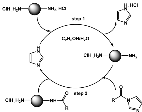
Scheme 2. Mechanism of Monoacylation
