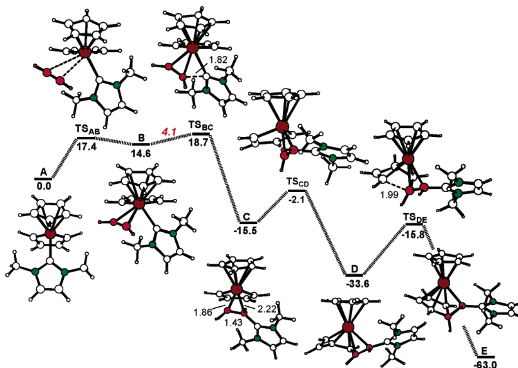
Figure 2. Reaction profile of the computed relative Gibbs free energies (in kcal/mol) for the reaction of the ruthenacyclopentatriene (A) with acetylene to give the formal [2 + 2 + 1] cycloaddition product (E) (bond distances in Å) with 1,3-dimethylimidazol-2-ylidene as the model NHC ligand.
