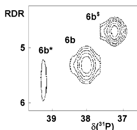
Figure 7. ^{31}\text{P} DOSY spectrum [243 MHz, relaxation delay 2.5 s, 0 °C, \text{CDCl}_3 solution] of an equilibrium mixture of 6b , 6b* , and 6b s . RDR = relative diffusion rate.
