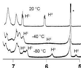
Figure 11. Variable-temperature 1 H NMR spectra [400 MHz] of a mixture of macrocyclic complex 5a and [2]catenane complex 5a* in CD 2 Cl 2 solution. The peak marked * is due to CHDCl 2 .
