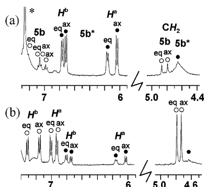
Figure 8. ^1\text{H} NMR spectra [400 MHz, 25 °C] of an equilibrium mixture of the macrocyclic complex 5b (○) and the [2]catenane 5b* (●) showing resonances assigned to axial (ax) and equatorial (eq) \text{C}_6\text{H}_4 and \text{OCH}_2 substituents: (a) spectrum in concentrated solution in \text{CDCl}_3 , when the [2]catenane 5b* is dominant (peak labeled * is due to \text{CHCl}_3 ); (b) spectrum in more dilute solution in \text{CD}_2\text{Cl}_2 , when 5b is dominant.
