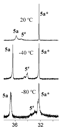
Figure 10. Variable-temperature 31 P NMR spectra [162 MHz, CD 2 -Cl 2 solution] of a mixture of isomers 5a , 5a* , and 5a# .
