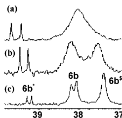
Figure 6. Variable-temperature ^{31}\text{P} NMR spectra [243 MHz, \text{CDCl}_3 solution] of the macrocyclic complex 6b , in equilibrium with the [2]catenane 6b* and double-ring isomers 6b S : (a) 60 °C; (b) 25 °C; (c) 0 °C.
