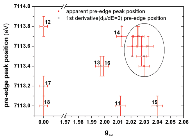
Figure 11. Diagram of XAS pre-edge energy vs isotropic g tensor of EPR for complexes 1 , 2 , 5 , [(\text{NO})_2\text{Fe}(\text{SET})_2]^- ( 6 ), [(\text{NO})_2\text{Fe}(\text{SCH}_2\text{C}(\equiv\text{O})\text{NHCH}_3)_2]^- ( 7 ), [(\text{NO})_2\text{Fe}(\text{SPh})_2]^- ( 8 ), [(\text{NO})_2\text{FeS}_3]^- ( 9 ), [(\text{NO})_2\text{Fe}(\text{SePh})_2]^- ( 10 ), [(\text{NO})\text{Fe}(\text{SPh})_3]^- ( 11 ), [(\text{NO})_2\text{Fe}(\mu\text{-SET})_2]^- ( 12 ), [(\text{NO})_2\text{Fe}(\mu\text{-SET})_2]^- ( 13 ), [(1\text{-Melm})_2(\eta^2\text{-ONO})\text{Fe}(\text{NO})_2] ( 14 ), [(\text{NO})\text{Fe}(\text{S}_2\text{CNET}_2)_2] ( 15 ), [(\text{NO})\text{Fe}(\text{S}_2\text{C}_6\text{H}_4)_2]_3 ( 16 ), [(\text{NO})\text{Fe}(\text{S}_2\text{C}_6\text{H}_4)_2]_3^+ ( 17 ), and [(\text{NO})\text{Fe}(\text{S},\text{S}-\text{C}_6\text{H}_4)_2]^- ( 18 ).
