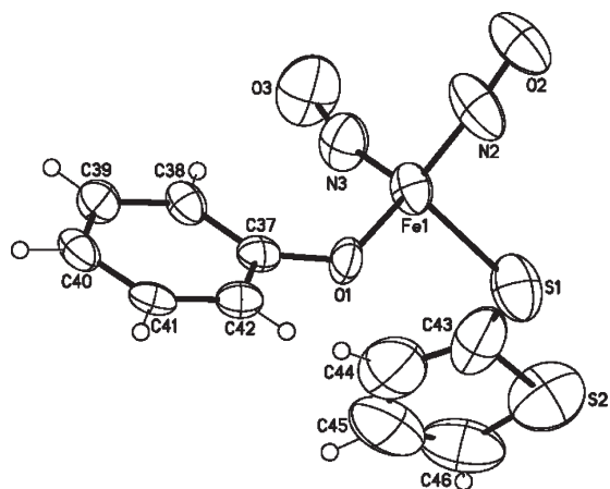
Figure 8. ORTEP drawing and labeling scheme of complex 4 with thermal ellipsoids drawn at 30% probability. Selected bond distances (Å) and angles (deg): Fe(1)–N(2) 1.686(4), Fe(1)–N(3) 1.683(4), Fe(1)–O(1) 1.960(3), Fe(1)–S(1) 2.286(2), N(2)–O(2) 1.144(6), N(3)–O(3) 1.185(5), N(2)–Fe(1)–N(3) 111.9(2), N(3)–Fe(1)–O(1) 115.5(1), N(2)–Fe(1)–O(1) 108.2(1), N(3)–Fe(1)–S(1) 110.6(1), N(2)–Fe(1)–S(1) 104.3(2), O(1)–Fe(1)–S(1) 105.6(1), O(2)–N(2)–Fe(1) 167.3(6), O(3)–N(3)–Fe(1) 164.3(4).
