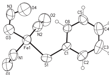
Figure 9. ORTEP drawing and labeling scheme of complex 6 with thermal ellipsoids drawn at 50% probability. Selected bond distances (Å) and angles (deg): Fe(1)–N(1) 1.686(6), Fe(1)–N(2) 1.641(6), Fe(1)–S(1) 2.231(2), Fe(1)–O(3) 2.043(6), N(1)–O(1) 1.157(6), N(2)–O(2) 1.176(6), N(3)–O(3) 1.186(7), N(3)–O(4) 1.100(1), Fe(1)–N(1)–O(1) 162.8(5), Fe(1)–N(2)–O(2) 165.7(5), O(3)–Fe(1)–S(1) 110.8(2).
