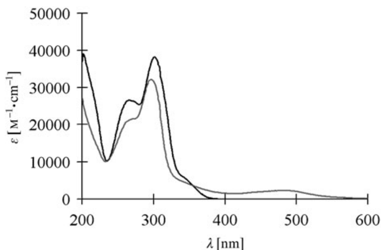
Fig. 1. UV/VIS Spectra (MeOH) of [\text{Ni}(\mathbf{2})_3]^{2+} (black line) and [\text{Fe}(\mathbf{2})_3]^{2+} (grey line) showing the band at 350 nm indicating complexation of the ligand and the MLCT transition at 485 nm for the \text{Fe}^{\text{II}} complex
