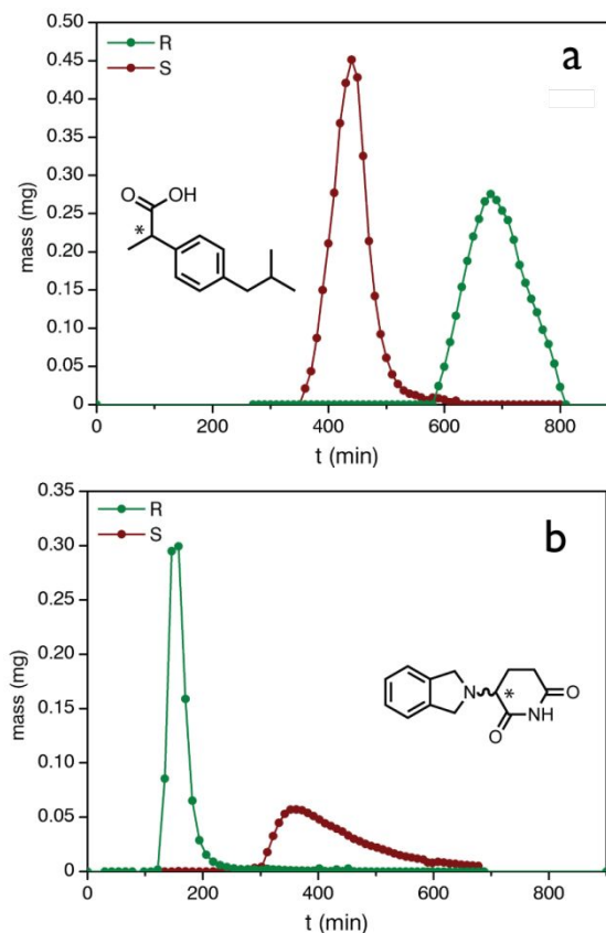
Figure 2. Gravity chromatographic separations at room temperature with a glass TAMOF-1 column with 100% acetonitrile as the mobile phase: (a) of (±)-ibuprofen; (b) (±)-thalidomide.
