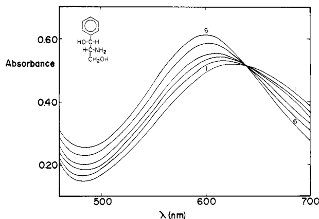
Figure 2. Absorption spectrum of [\text{CuSalPAHP}]_2 \cdot \text{H}_2\text{O} ( 1.45 \times 10^{-3} M) in the presence of (+)-PAHP in ethanol. Concentrations of (+)-PAHP: (1) 0; (2) 1.46 \times 10^{-3} M; (3) 2.92 \times 10^{-3} M; (4) 4.38 \times 10^{-3} M; (5) 7.30 \times 10^{-3} M; (6) 1.02 \times 10^{-2} M.
