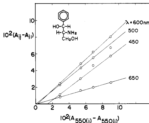
Figure 3. Test of spectral data for two absorbing species in the [\text{CuSalPAHP}]_2 \cdot \text{H}_2\text{O} -(+)-PAHP system.
