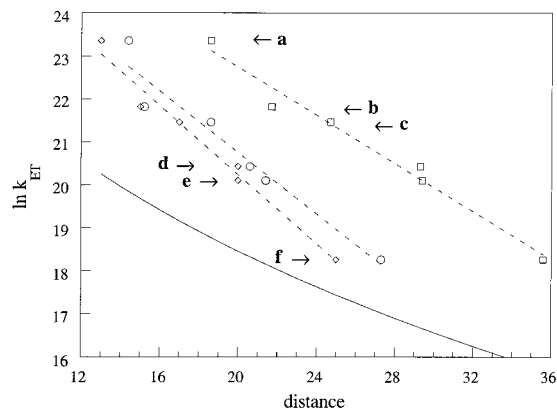
Figure 3. Distance dependence of ET rates in dimeric Zn,Fe porphyrins 12a–f : d_{\text{space}} (○), d_{\text{bond}} (□), N_{\text{bond}} (◇), eq 5, with R = d_{\text{space}} + 6.97 \text{\AA} (—).
