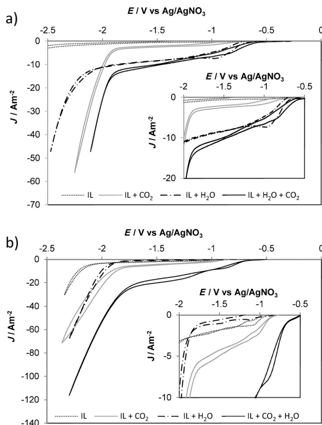
Figure 1. Cyclic voltammograms recorded with a silver working electrode in acetonitrile solutions with 0.1 \text{ mol L}^{-1} of the ionic liquids (IL) a) [\text{P}_{66614}][\text{NTf}_2] and b) [\text{P}_{66614}][124\text{Triz}] . Inset: magnified sections.
