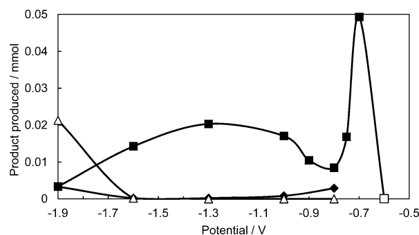
Figure 2. Variation of product yield as a function of applied potential vs Ag/AgNO 3 after 10 C of charge is passed using a CO 2 saturated hydrated (0.7 mol L −1 ) 0.1 mol L −1 [P 66614 ][124Triz] in MeCN electrolyte at a Ag electrode. (■ formate, ♦ CO, △ H 2 ). Note the formate generated at −0.6 V (□) was obtained following 24 h of electrolysis during which only 1.5 C of charge had passed.
