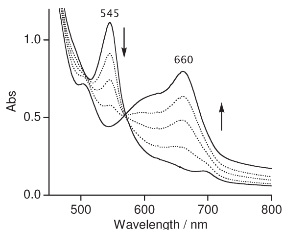
Figure 3. Absorption spectral change for electrochemical oxidation of (TMP)Fe IV O at 1.10 V vs SCE in dichloromethane containing 0.1 M tetra- n -butylammonium perchlorate at -60^{\circ}\text{C} . Experimental conditions are described in the Experimental Section.
