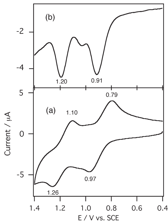
Figure 2. (a) Cyclic voltammogram and (b) differential pulse voltammogram of (TMP)Fe IV O in dichloromethane containing 0.1 M tetra- n -butylammonium perchlorate at -60^\circ\text{C} . The scan rate was 100 mV/s.
