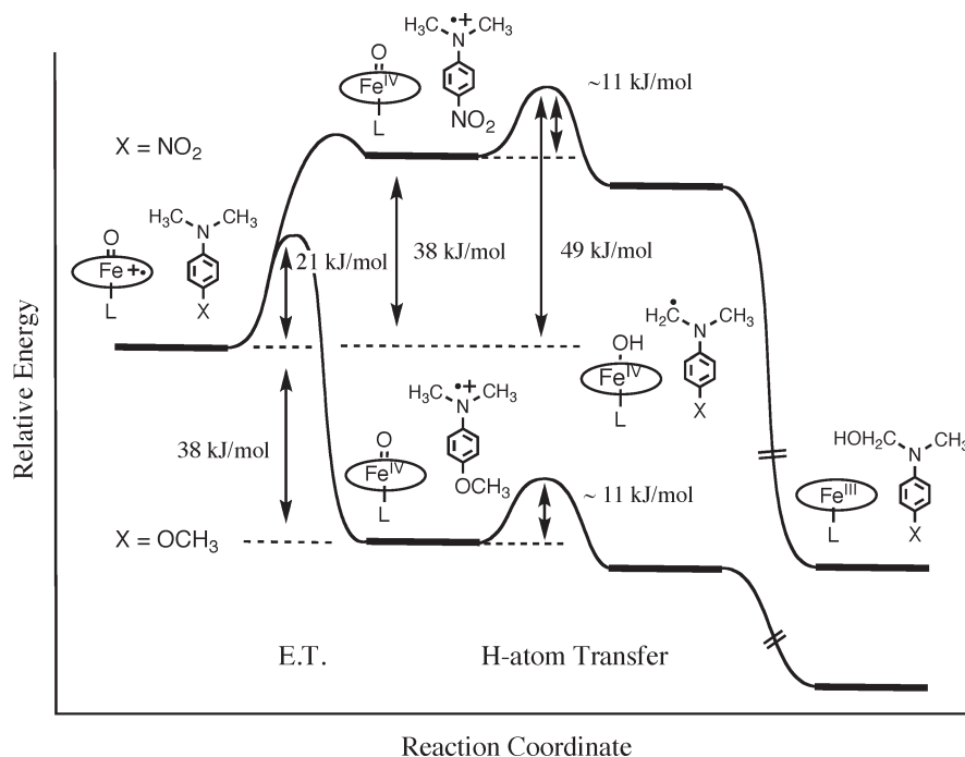
Figure 5. Reaction coordinate diagram showing the reaction profile for the demethylation of N,N -dimethyl- p -nitroaniline and N,N -dimethyl- p -methoxyaniline with (\text{TMP}^{+\bullet})\text{Fe}^{\text{IV}}\text{O}(\text{L}) . The structure of the H-atom transferred complex and the relative energies of the H-atom transferred complex and the final products are uncertain.
