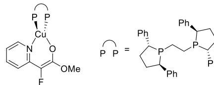
b. The studied complex derived from [Cu]/( R,R )-BPE and substrate 1a
