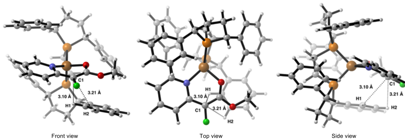
d. Optimized structure of Cu-control and Cu-1 in a quadrant diagram
