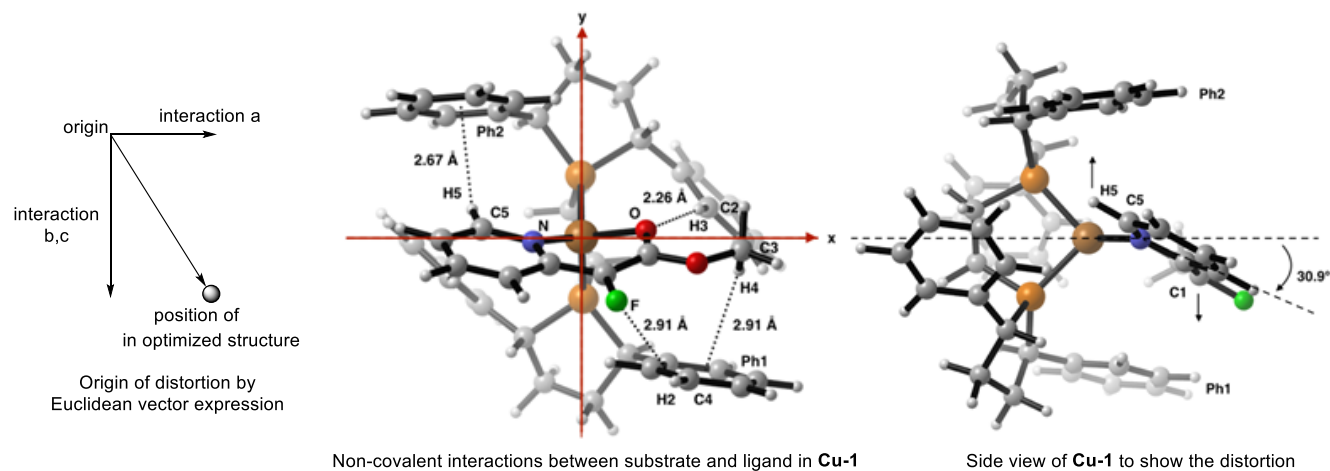
Non-covalent interactions between substrate and ligand in Cu-1
