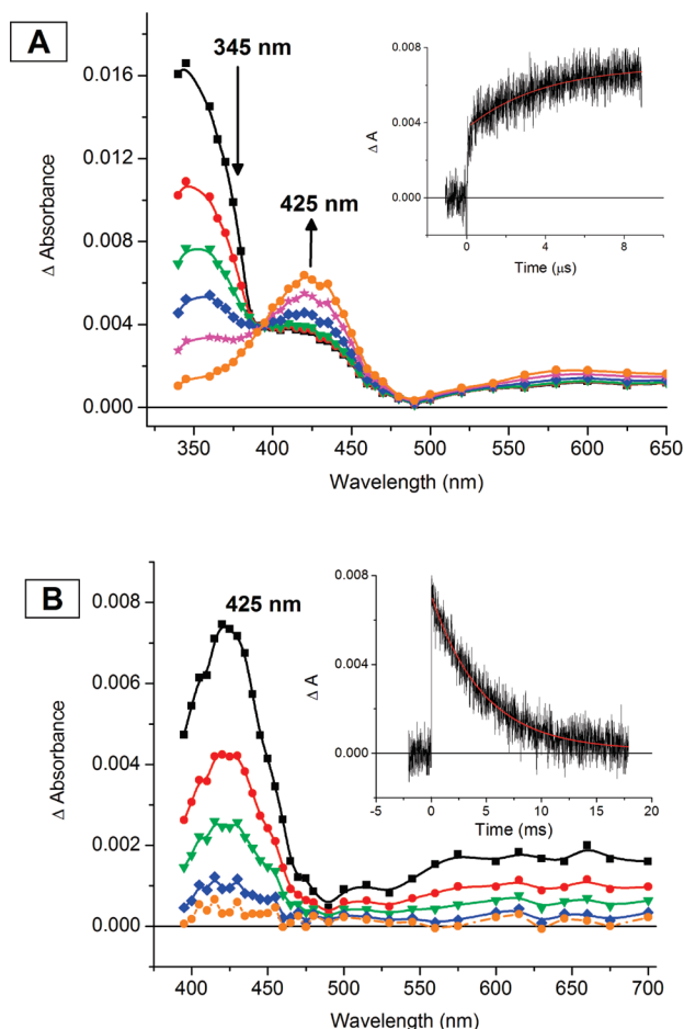
Figure 6. Absorption difference spectra [ \text{NM}_{\text{e}_2}\text{LCu}^{\text{II}}\text{-X} - \text{NM}_{\text{e}_2}\text{LCu}^{\text{I}}\text{-CO} ] recorded after pulsed \lambda_{\text{ex}} = 355 nm excitation of \text{NM}_{\text{e}_2}\text{LCu}^{\text{I}}\text{-CO} in THF at 193 K under 1 atm \text{O}_2\text{:CO} (1:1) mixture. The spectra were recorded at various delay times: (A) 0–5 \mu\text{s} , representing the conversion of \text{NM}_{\text{e}_2}\text{LCu}^{\text{I}} to a mixture of \text{NM}_{\text{e}_2}\text{LCu}^{\text{I}}\text{-CO} and \text{NM}_{\text{e}_2}\text{LCu}^{\text{II}}\text{-O}_2^- (black squares, 0 \mu\text{s} ; red circles, 0.1 \mu\text{s} ; green triangles, 0.25 \mu\text{s} ; blue diamonds, 1 \mu\text{s} ; magenta stars, 2.5 \mu\text{s} ; orange circles, 5.0 \mu\text{s} ). The inset is an absorption transient monitored at 425 nm with a superimposed first-order fit (in red), k_{\text{obs}} = 2.92 \times 10^5 \text{ s}^{-1} . (B) 0–20 ms, representing the conversion from \text{NM}_{\text{e}_2}\text{LCu}^{\text{II}}\text{-O}_2^- to \text{NM}_{\text{e}_2}\text{LCu}^{\text{I}}\text{-CO} (black squares, 0 ms; red circles, 2.5 ms; green triangles, 5.0 ms; blue diamonds, 10 ms; orange circles, 20 ms). The inset is an absorption transient monitored at 425 nm with a superimposed first-order fit (in red), k_{\text{obs}} = 236 \text{ s}^{-1} .
