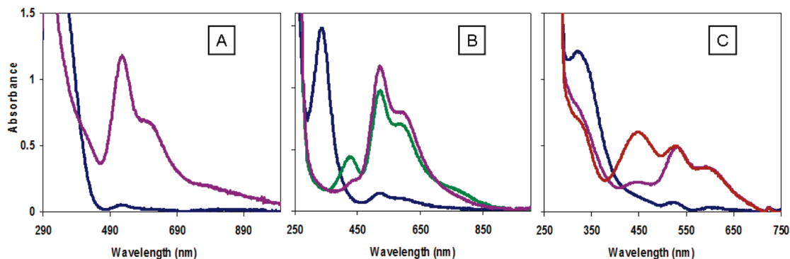
Figure 7. UV–visible spectra in MeTHF at -128\text{ }^{\circ}\text{C} representing \text{O}_2 + {}^{\text{P}}\text{LCu}^{\text{I}} (dark blue) to yield (A) [\{({}^{\text{tmpa}}\text{L})\text{Cu}^{\text{II}}\}_2(\text{O}_2^{2-})]^{2+} (purple); (B) {}^{\text{P}}\text{LCu}^{\text{II}}\text{-O}_2^- (green) and [\{({}^{\text{P}}\text{L})\text{Cu}^{\text{II}}\}_2(\text{O}_2^{2-})]^{2+} (purple); and (C) [\{({}^{\text{NMe}_2}\text{L})\text{Cu}^{\text{II}}\}_2(\text{O}_2^{2-})]^{2+} (purple) and a new copper–dioxygen adduct of {}^{\text{NMe}_2}\text{L} (brown).
