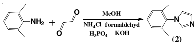
Scheme-II: Synthesis reaction of 1-(2,6-dimethylphenyl)-1H-imidazole (2)
