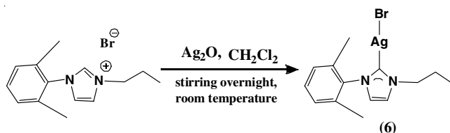
Scheme-VI: Synthesis of silver complex [\text{Ag}(\text{NHC})\text{Br}] (6)
