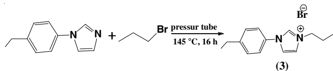
Scheme-III: Synthesis reaction of imidazolium salt (3)
