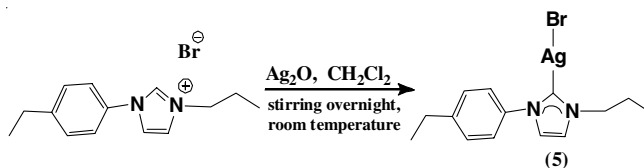
Scheme-V: Synthesis of silver complex [\text{Ag}(\text{NHC})\text{Br}] (5)
