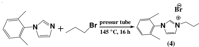
Scheme-IV: Synthesis reaction of imidazolium salt (4)
