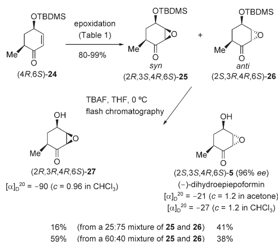
Scheme 4. Epoxidation of cyclohexenone (4 R ,6 S )- 24 and completion of the synthesis of (–)- 27 and (–)-dihydroepiopoformin ( 5 ).
