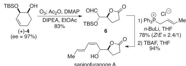
Scheme 3. Synthesis of Sapinofuranone A
