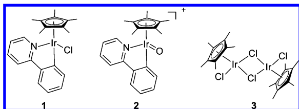
Figure 1. Cp*Ir complexes for C–H hydroxylation.
