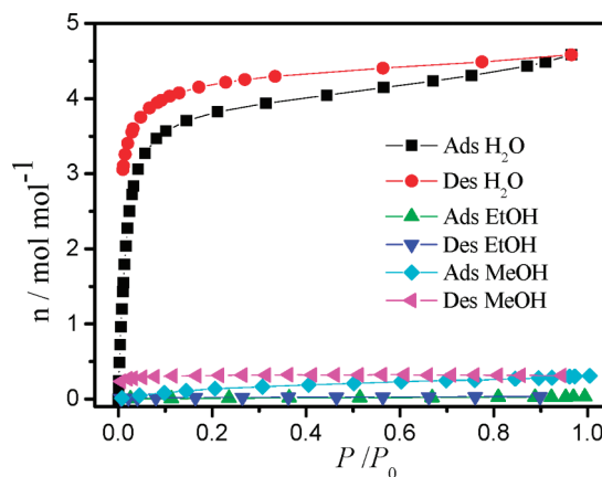
Figure 4. Solvent vapor adsorption and desorption isotherms of 2 at 298 K, which shows highly selective adsorption of H 2 O vapor over other organic solvents.
