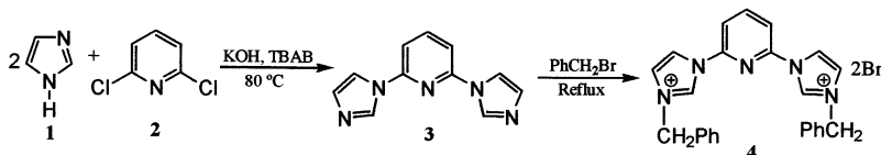
Scheme 1. Synthesis of 1,1'-(pyridine-2,6-diyl)bis(3-benzyl-1H-imidazolium) bromide.
