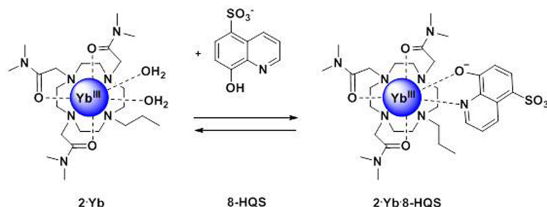
Scheme 1. Formation of the 1:1 Ternary Complex between 2·Yb and 8-HQS
