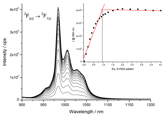
Figure 2. Evolution of the Yb(III) NIR emission ( \lambda_{\text{ex}} = 360\text{ nm} ) of 2·Yb ( 5 \times 10^{-5} M) in HEPES buffer upon addition of 8-HQS .
