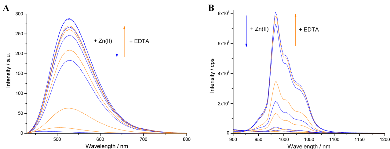
Figure 8. Evolution of the fluorescence (A) and NIR emission (B) of 2-Yb·8-HQS ( 5 \times 10^{-5} M) in HEPES buffer upon titration with Zn(II) (blue curves; 0→10 equiv) followed by the addition of EDTA (orange curves; 0→10 equiv).
