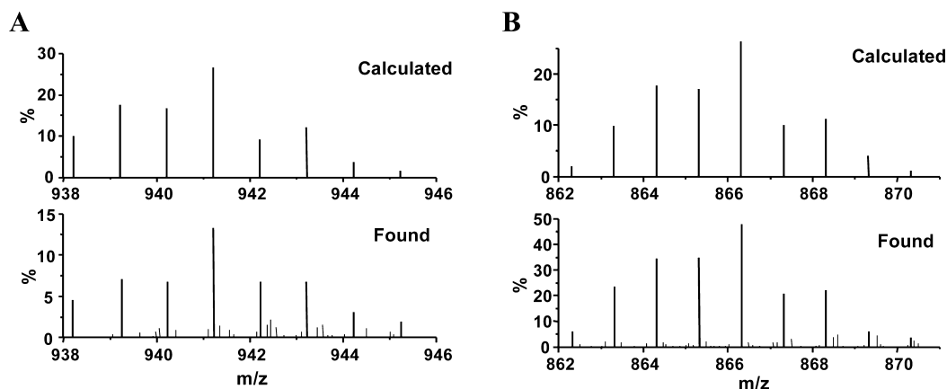
Figure 1. Parts of the MALDI mass spectra of 2·Yb ( 10^{-4} M in methanol) in the absence (A) and presence of 8-HQS (B) and their corresponding calculated isotopic distribution patterns.
