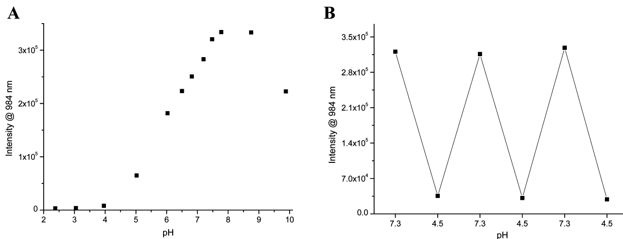
Figure 5. (A) Effect of the pH on the metal-centered emission intensity of a 1:1 2-Yb-8-HQS solution in 0.1 M NaCl; [2\text{-Yb}] = [8\text{-HQS}] = 5 \times 10^{-5} M, \lambda_{\text{ex}} = 360 nm and \lambda_{\text{an}} = 984 nm. (B) Reversibility of the ON-OFF switching behavior of the metal-centered emission as a function of the pH.
