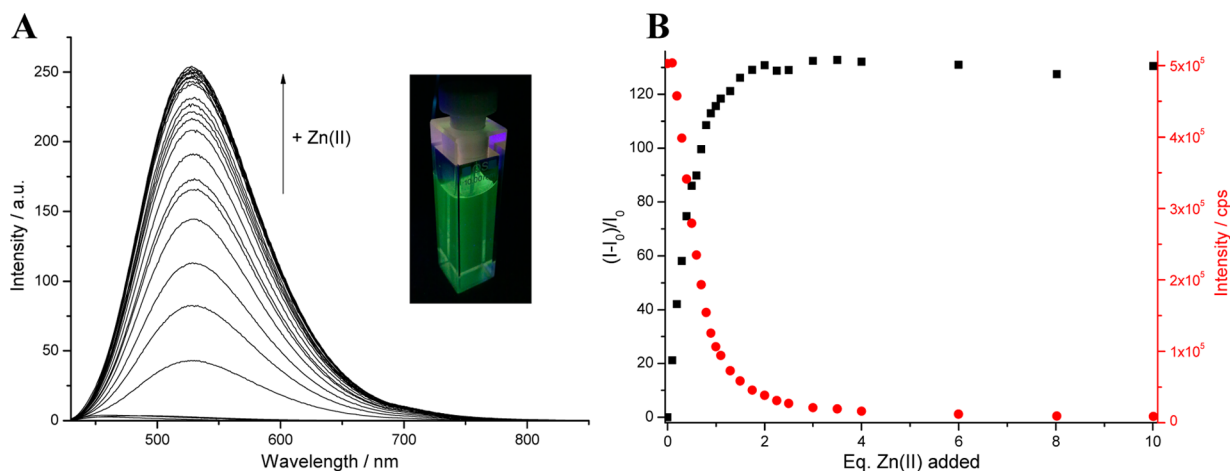
Figure 4. (A) Evolution of the fluorescence emission spectrum ( \lambda_{\text{ex}} = 360 nm) of 2-Yb-8-HQS ( 5 \times 10^{-5} M) in HEPES buffer upon titration with Zn(II). Inset: The emission arising from a solution of 2-Yb-8-HQS in the presence of Zn(II) under a UV–visible lamp ( \lambda_{\text{ex}} = 365 nm). (B) The fluorescence enhancement, (I - I_0)/I_0 , observed in the visible region (black squares) and the concomitant quenching of the Yb-centered NIR emission (right y-scale, red circles) vs the equivalents of Zn(II) added.
