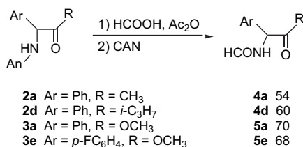
Scheme 3. Formylation and oxidation with CAN of acylated products 2 and 3 .
