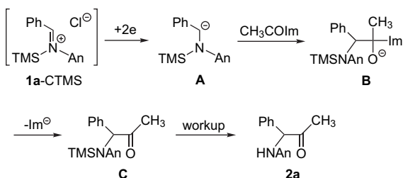
Scheme 4. Reaction mechanism.
