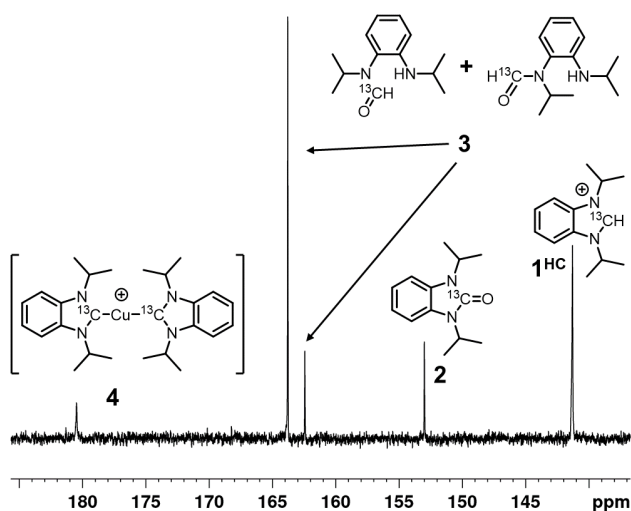
Figure 4. Quantitative IG- ^{13}\text{C}\{^1\text{H}\} NMR spectra of the supernatants obtained from \text{CuO}_x etching experiments using ^{13}\text{C} -labelled 1^{\text{Hc}} . \text{Cu}^{(0)} etching is given in the supporting information. Yields are given in Table 1, entries 3-4.
