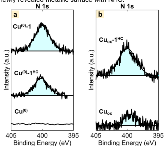
Figure 2. (a) Stacked N 1s XPS illustrating the functionalization of Cu 0 surfaces with NHC 1 and NHC precursor 1 HC , and (b) N 1s XPS plots illustrating the sample after treatment of Cu ox surfaces with NHC precursor 1 HC . In both cases, treatment was accomplished with 10 mM DCE solutions of the hydrogen carbonate salt 1 HC or free NHC 1. [16]
