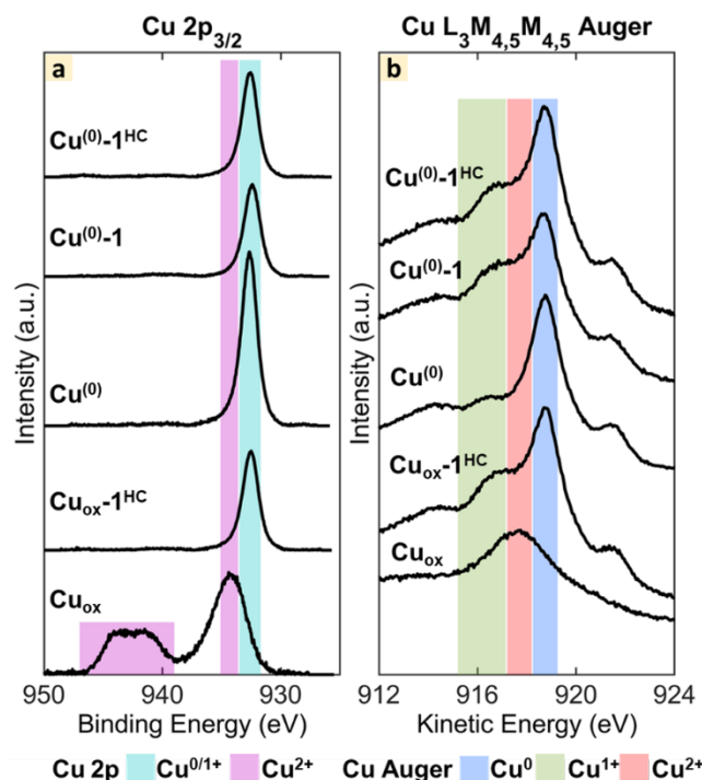
Figure 1. Stacked Cu 2p 3/2 XPS (a) and Cu LMM Auger (b) plots illustrating the removal of metal oxides by treating cleaned (Cu 0 ) and oxidized (Cu ox ) copper surfaces with solutions of the free NHC 1 or its hydrogen carbonate salt 1 HC .
