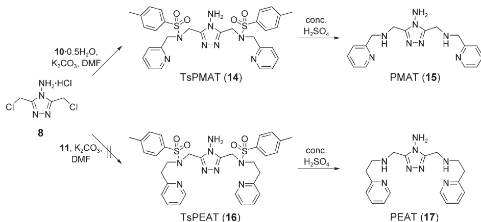
Scheme 4. Synthesis of 4-amino-3,5-bis([ N -(2-pyridylmethyl)- N -(4-toluenesulfonyl)amino]methyl)-4H-1,2,4-triazole (TsPMAT, 14 ) and 4-amino-3,5-bis([ N -(2-pyridylmethyl)amino]methyl)-4H-1,2,4-triazole (PMAT, 15 ) and attempted synthesis of 4-amino-3,5-bis([ N -[2-(2-pyridyl)ethyl]- N -(4-toluenesulfonyl)amino]methyl)-4H-1,2,4-triazole (TsPEAT, 16 ) and 4-amino-3,5-bis([ N -[2-(2-pyridyl)ethyl]amino]methyl)-4H-1,2,4-triazole (PEAT, 17 ).
