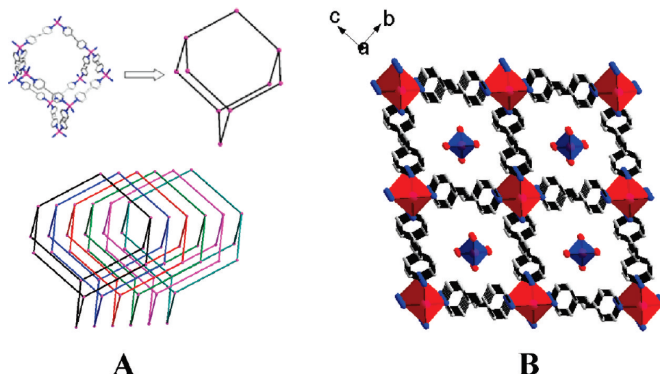
Figure 9. (A) Simplified view of a single diamond-type \text{Ag(dpa)}_2^+ network, upper, and the 6-fold interpenetration of the same diamond-type net in \text{Ag(dpa)}_2\text{ReO}_4 ( 9 ), lower. Each node represents a Ag atom. (B) An \sim[100] polyhedral view of 9 , with red polyhedra = Ag-centered tetrahedra and blue polyhedra = \text{ReO}_4^- .
