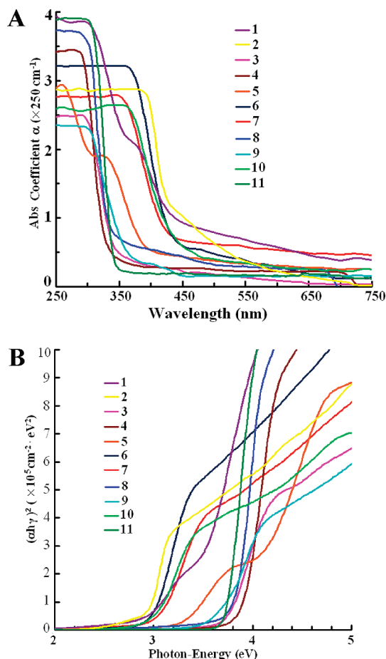
Figure 10. (A) A plot of the optical absorption coefficients, \alpha ( \text{cm}^{-1} ) versus wavelength (nm), and (B) a plot of (\alpha h\nu)^2 vs h\nu for hybrids 1–9, 10 (AgReO 4 (pyz)), and 11 (AgReO 4 ).
