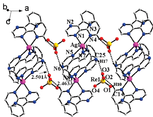
Figure 1. Structural view of 1 , \text{Ag}(\text{bpp})_2\text{ReO}_4 , with hydrogen bonds drawn as dashed lines and symmetry-unique atom types labeled. Hydrogen atoms are omitted for clarity.
