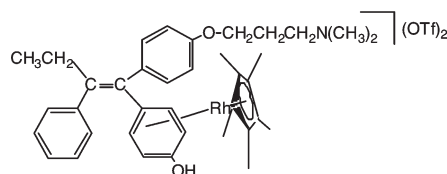
trans -7
