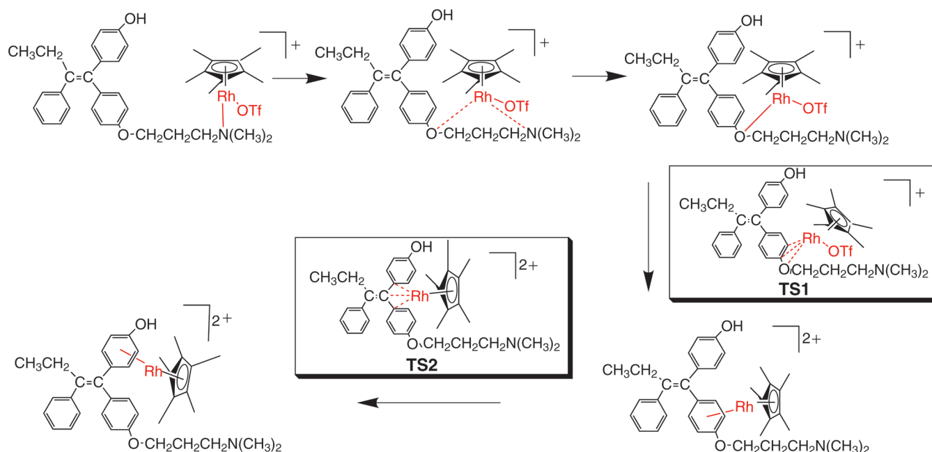
Scheme 1. Plausible Reaction Mechanism for the N- \pi Rearrangement a
