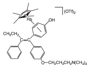
cis -6
