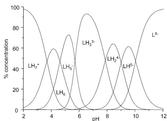
Figure 2. Distribution curves of the ligand computed from the pK_a values at pH 2–12.
