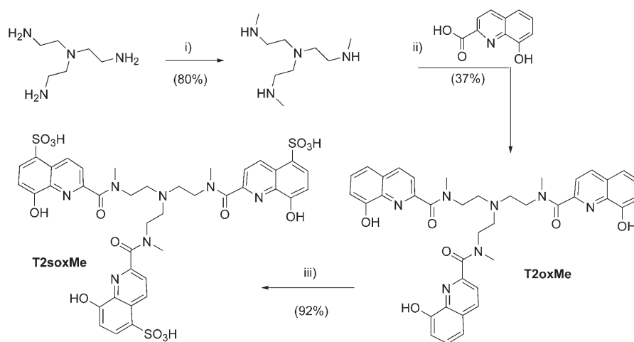
Scheme 1. Synthetic pathway used to obtain ligand T2soxMe : i) a) \text{EtCO}_2\text{Cl} , \text{H}_2\text{O} , toluene; b) \text{LiAlH}_4 , THF; ii) 2-carboxy-8-hydroxyquinoline, N,N' -carbonyl diimidazole (CDI), THF; iii) \text{H}_2\text{SO}_4 , \text{SO}_3 (20%).
