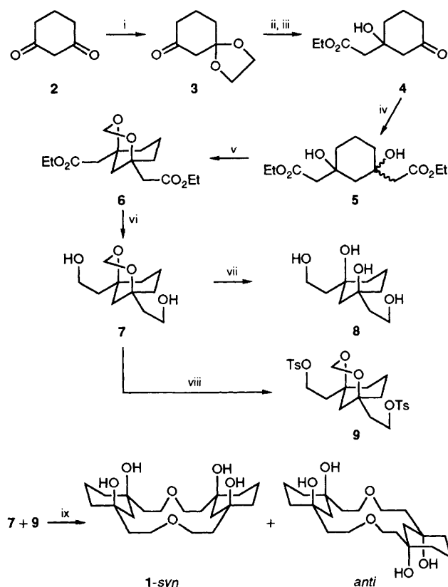
Scheme 1 Reagents and conditions: i, ethyleneglycol, p -TsOH (Ts = p -MeC 6 H 4 SO 2 ), 53%; ii, MeCO 2 Et, LDA, H + ; iii, H + , 74%; iv, MeCO 2 Et, LDA, H + ; 94% ( cis-trans = 1:1 mixture); v, (CH 2 O) n , p -TsOH, EtOH, 48%; vi, LiAlH 4 , H + , quant.; vii, H + , 84%; viii, p -TsOH, quant.; ix, CsOH, H + , 2.3%
