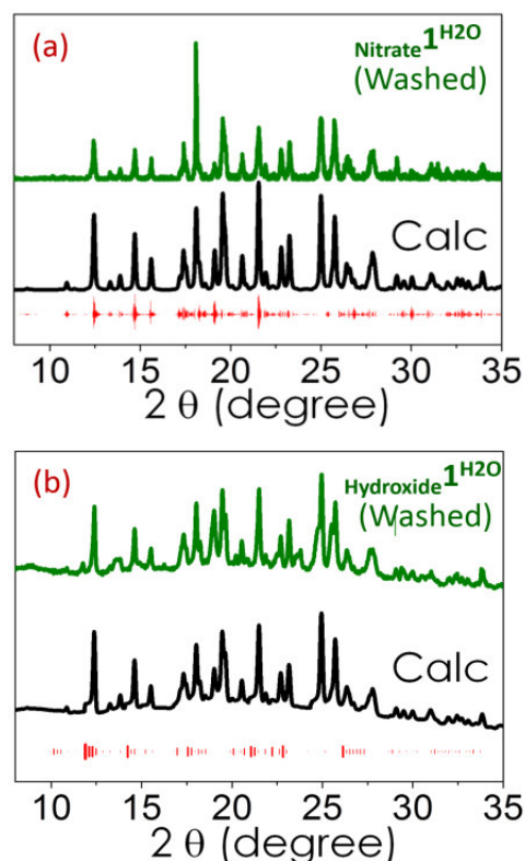
Fig. 7. Comparison between the simulated PXRD pattern of \mathbf{1} and experimental patterns recorded for the methanol washed Nitrate \mathbf{1}^{\text{H}_2\text{O}} (a) and Hydroxide \mathbf{1}^{\text{H}_2\text{O}} (b), indicating that the washing significantly improved the phase purity. The difference between the simulated and experimental patterns is plotted in red.
