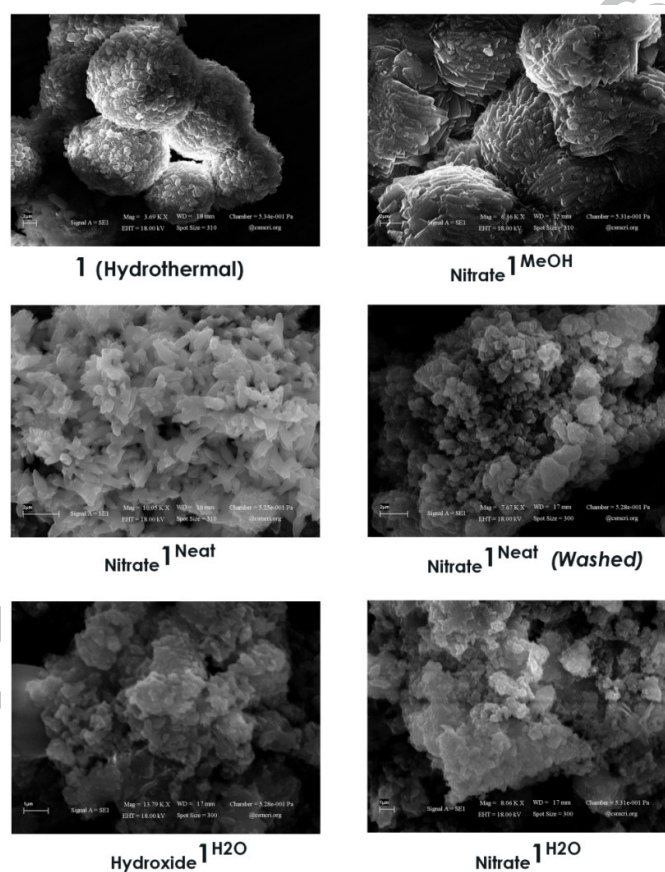
Fig. 8. SEM micrographs of Co CP, 1 prepared via different synthetic methodologies. The morphological resemblance between 1 (hydrothermal) and Nitrate 1 MeOH is noteworthy.
