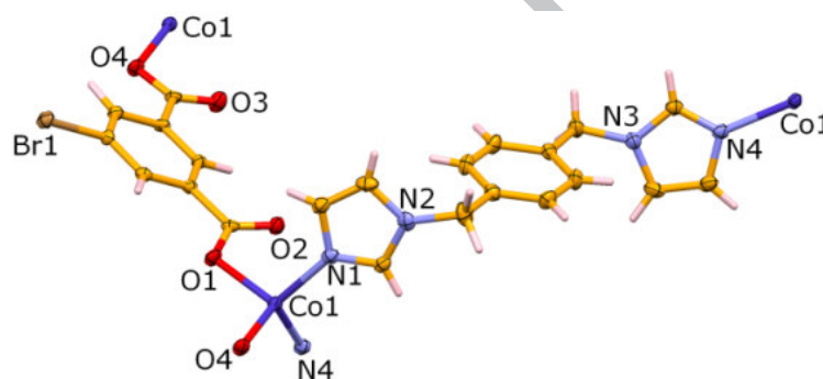
Fig. 1. ORTEP diagram depicting the coordination sphere with the atom numbering scheme for 1 (50% probability factor for the thermal ellipsoids).
