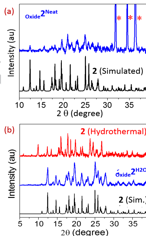
Fig. 5. A comparison between the simulated PXRD patterns of 2 and experimental patterns of Oxide 2 Neat indicate the presence of ZnO (reflections marked with an asterisk) as an impurity in
