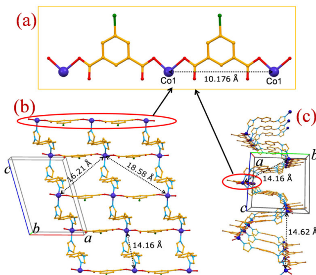
Fig. 2. (a) \{\text{Co(II)BrIP}\}_n chain running along the a -axis; (b) sql type [\text{Co}(\text{BrIP})(\text{BIX})]_n network with 16.21 \times 18.58 \text{ \AA}^2 windows through which another such network interpenetrates; (c) deep undulated network constructed upon strategic connections between diagonal glide related \{\text{Co(II)BrIP}\}_n chains via BIX molecules confined in an anti -conformation.
