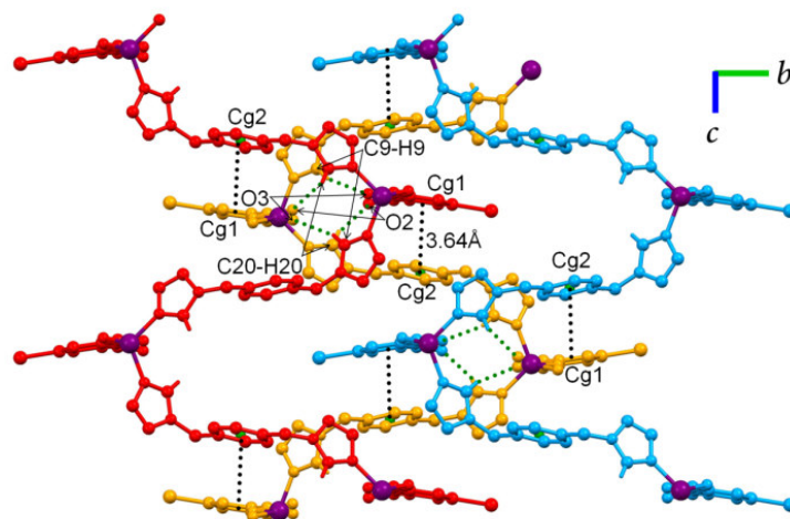
Fig. 4. Close-up view along the a -axis depicting three interlocked [\text{Co}(\text{BrIP})(\text{BIX})]_n networks glued together by means of C–H···O hydrogen bonding and \pi\cdots\pi interactions between the phenyl rings of BrIP and BIX .
