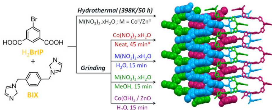
Scheme 1. Hydrothermal and various grinding reactions between the ligands ( \text{H}_2\text{BrIP} / \text{BIX} ) and metal precursors yield the interpenetrated ternary coordination polymers 1 and 2 .
