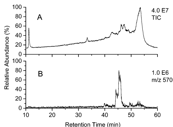
FIGURE 5. Reversed phase LC-MS analysis of products derived from Fe(II)-mediated autooxidation of linoleic acid in the presence of N -benzoyl-L-histidine. (A) TIC; (B) SIC for \text{MH}^+ ( m/z 570) expected for EKODE ( M_w = 310 ) Michael adducts.
