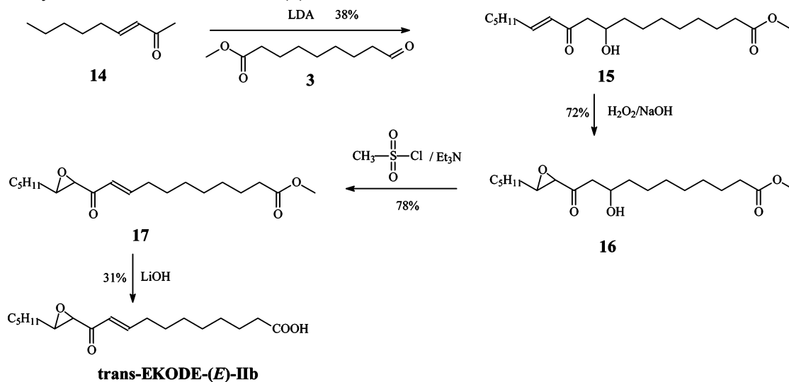
SCHEME 3. Synthetic Route to trans -EKODE-( E )-IIb
