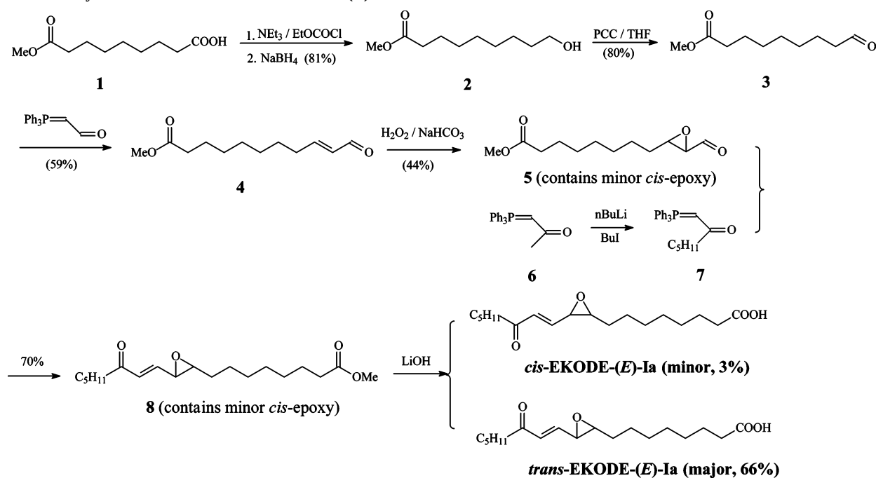
SCHEME 1. Synthetic Route to trans/cis -EKODE-(E)-Ia
