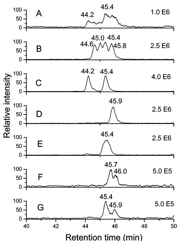
FIGURE 6. Reversed phase LC selected ion chromatograms for \text{MH}^+ ( m/z 570) of the N^\alpha -benzoyl-L-histidine adducts of (A) EKODE isomers derived from autooxidation of linoleic acid ( \text{Fe(II)/AH}_2 ); (B) trans -EKODE-IIb; (C) trans -EKODE-IIa; (D) trans -EKODE-Ib; (E) trans -EKODE-Ia; (F) cis -EKODE-Ib; and (G) cis -EKODE-Ia.
