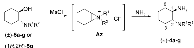
Scheme 3. The conversion of ( \pm )- trans -2-aminocyclohexanols 5 into racemic diamines ( \pm )- 4a–g proceeds through a meso -aziridininium ion intermediate ( Az ).
