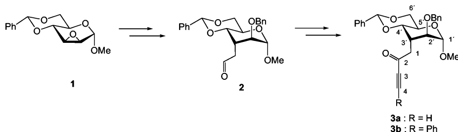
Scheme 1. 1-(Methyl 2- O -benzyl-4,6- O -benzylidene-3-deoxy- \alpha -D-altropyranosid-3-yl)but-3-yn-2-ones 3a , b .
