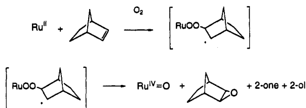
Scheme 1. Proposed Mechanism for Initiation of the Oxidation of Norbornene by [Ru(dmp) 2 (CH 3 CN) 2 ](PF 6 ) 2 and O 2
