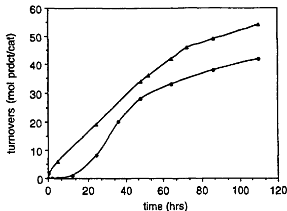
Figure 2. Oxidation of norbornene (0.6 M) in \text{CH}_3\text{CN} by 2 \times 10^{-4} \text{ M} ( 10^{-5} \text{ mol} ) of [\text{Ru}(\text{dmp})_2(\text{CH}_3\text{CN})_2](\text{PF}_6)_2 at 65^\circ\text{C} and 40 psig of \text{O}_2 (lower) and in the presence of 3 \times 10^{-5} \text{ mol} of 0.2 M \text{H}_2\text{O}_2 (upper).
