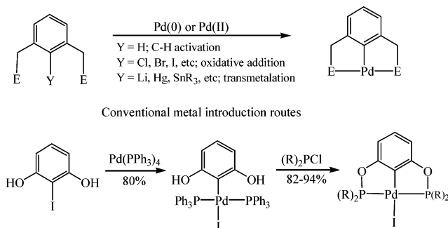
Uozumi's ligand introduction route for the synthesis of PCP pincer palladium complexes
