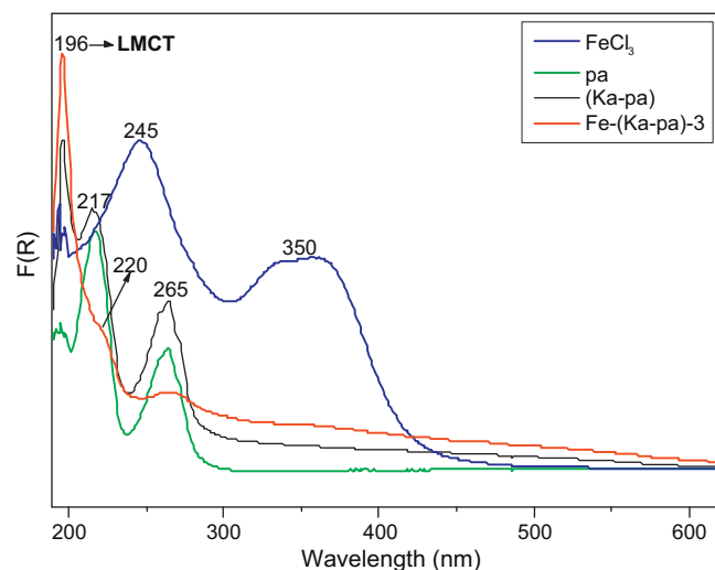
Fig. 6. UV/vis spectra of the compounds Fe(III) chloride, picolinic acid (pa), Ka-pa and Fe(Ka-pa)-3.
