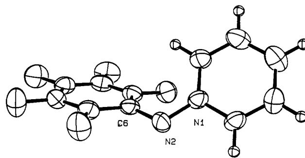
Figure 3. The crystal structure of ylide 9 .
