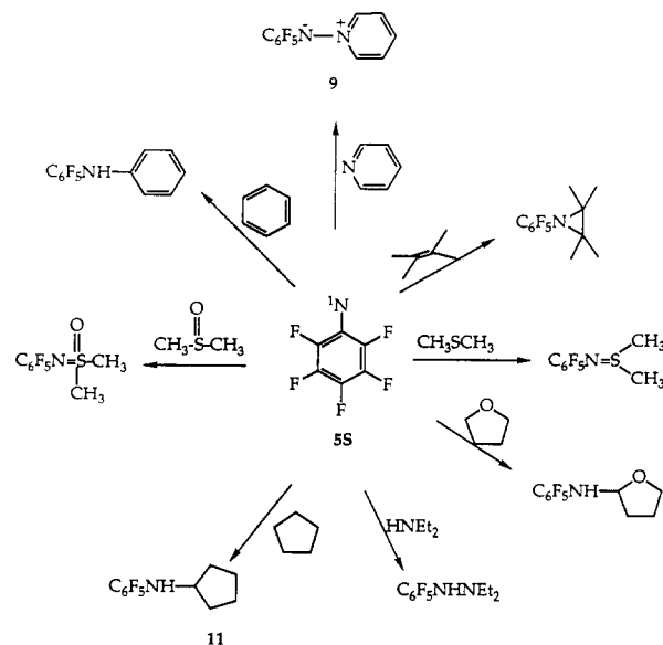
Figure 1. The products formed on photolysis of pentafluorophenylazide 4 in various solvents at ambient temperature.
