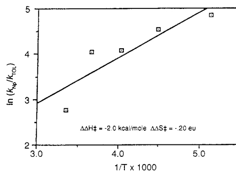
Figure 2. A logarithmic plot of the reactivity ratio of toluene/naphthalene towards \mathbf{5S} , versus temperature. -1
