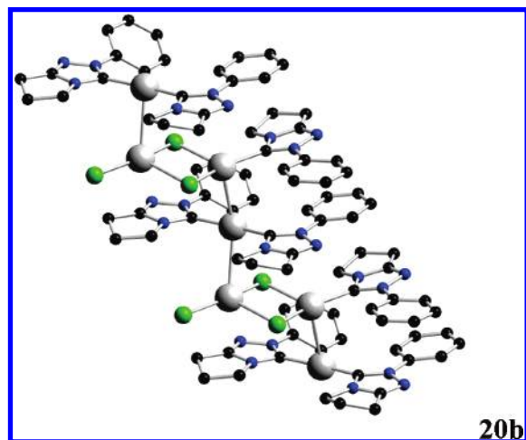
Figure 5. Ball-and-stick representations of complex (TPh)AgCl as a bridged Ag-( \mu\text{Cl}_2 )-Ag polymer ( 20b ). Hydrogen atoms have been omitted for clarity.
