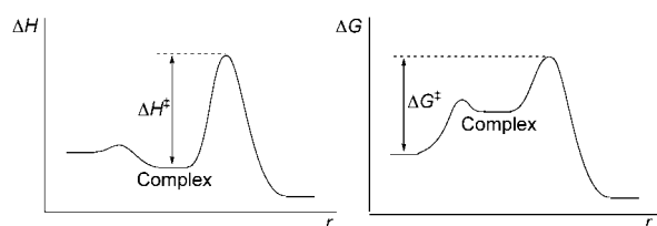
Figure 3. Transition state activation energies. Left: enthalpy, measured as the energy difference between the complex and the TS structure and, right: Gibbs energy measured as the energy difference between the reagents and the TS structures.
