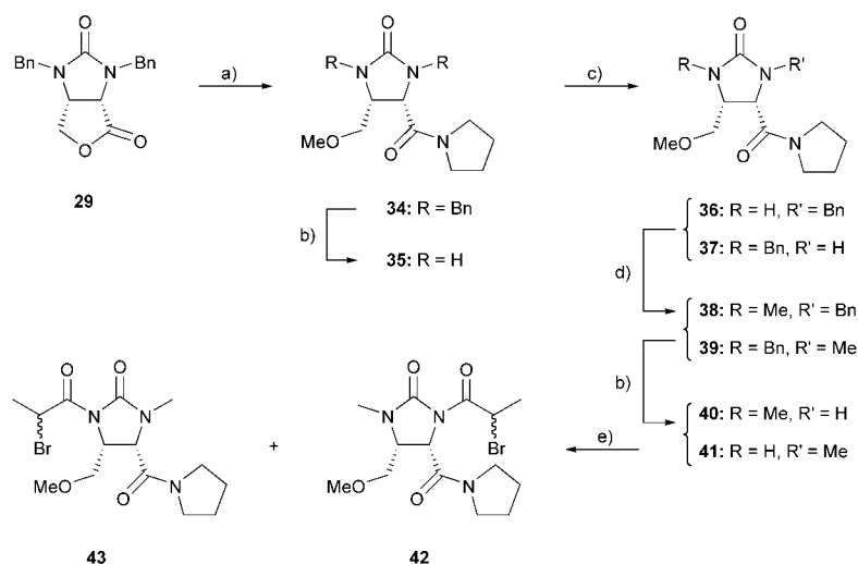
Scheme 7. Synthesis of the model substrate 42 . a) i) pyrrolidine (1.5 equiv), \text{CH}_2\text{Cl}_2 , rt, 24 h; ii) \text{AgO} (1.5 equiv), MeI (excess), MeCN, 40^\circ\text{C} , 3 d, 59%. b) \text{Pd/C} , \text{H}_2 , \text{HClO}_4 , MeOH, rt, quantitative. c) NaH (0.5 molequiv), BnBr (0.5 molequiv), THF, 0^\circ\text{C} to rt, 3 h, 35%. d) NaH (0.5 molequiv), MeI (1.0 equiv), THF, 0^\circ\text{C} to rt, 3 h, 91%. e) t\text{BuOK} (1.0 equiv), THF, MeCHBrCOBr (1.4 equiv), -50 to -30^\circ\text{C} , 87%.
