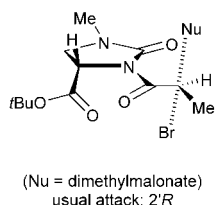
Figure 1. Reaction mechanism proposed by Nunami et al. [37–39] to explain their experimental observations.
