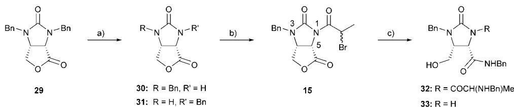
Scheme 6. Synthesis of the model substrate 15 and nucleophilic substitution attempts. a) Pd/C, H 2 , HClO 4 , MeOH, rt. b) 2,6-Lutidine, MeCHBrCOBr, CH 2 Cl 2 , –20 °C. c) Benzylamine (1.5 equiv), TEA (1.2 equiv), THF, rt, 48 h.
