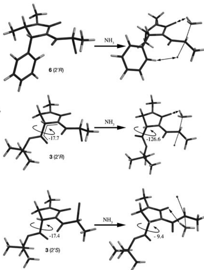
Figure 6. Transition state structures of compounds 3 (2' R ), (2' S ) and 6 (2' R ) at HF/6-31G**. Angles in degrees (the negative angles have the same meaning as in Figure 5).
