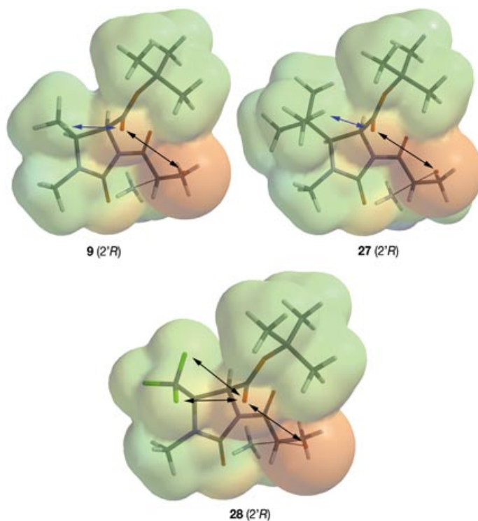
Figure 12. Electronic isodensity surfaces (0.002 e - au -3 , HF/6-31G**) mapped with the electrostatic potential, for TS structures of compounds 9 , 27 and 28 (2'R epimers), showing the electrostatic interactions (repulsive interactions: black arrows; attractive interactions: blue arrows) between the leaving bromide and the auxiliary substituent. Red zones indicate negative potential and blue zones indicate positive potential.
