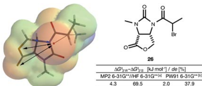
Figure 11. Theoretical expected performance of structure 26 as a chiral auxiliary in DKR reactions, showing the electrostatic interactions in the transition state of epimer 2'R (repulsive interactions: black arrows; attractive interactions: blue arrows). (Electronic isodensity surfaces ( 0.002 \text{ e}^- \text{ au}^{-3} , HF/6-31G**) mapped with the electrostatic potential. Red zones indicate negative potential and blue zones indicate positive potential.) Scaling factors: a = 1.58 and b = 1.78 .
