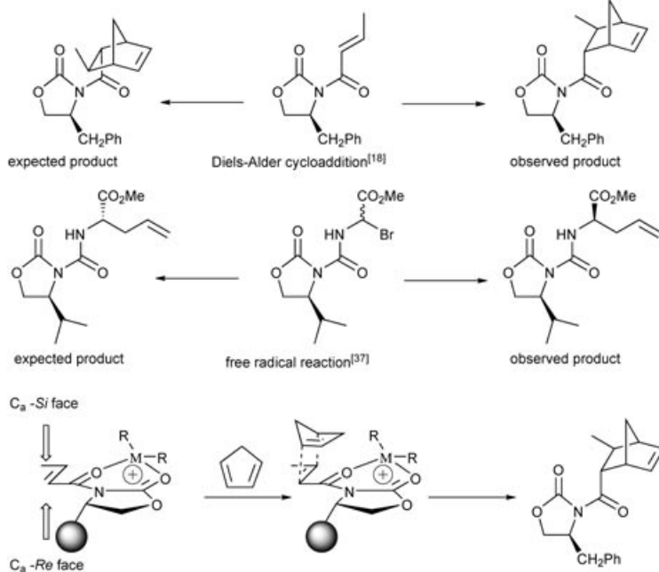
Scheme 2. Use of oxazolidinones as chiral auxiliaries in cycloadditions and in free radical reactions. Bottom: Mechanism proposed by Evans et al. [18] to explain their experimental results on cycloadditions.
