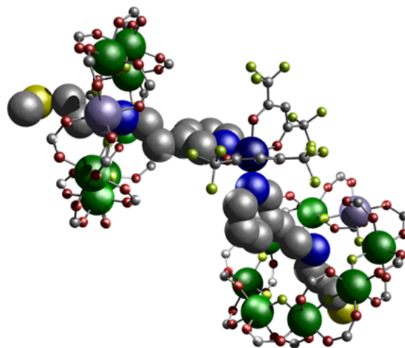
Figure 5. Crystal structure of 10 . Colors as for Figure 3.
