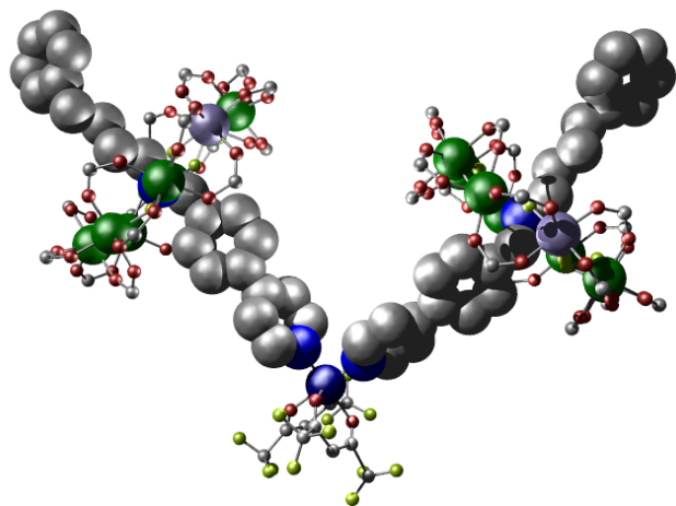
Figure 4. Crystal structure of 8 . Colors as for Figure 1.
