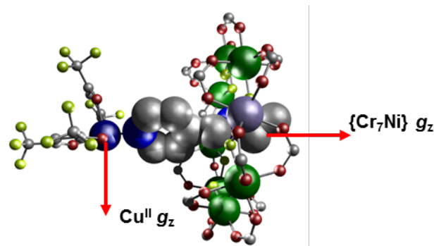
Figure 2. Crystal structure of 4 , the red arrows show the unique z axis for the \text{Cu}^{\text{II}} and \{\text{Cr}_7\text{Ni}\} . For 4 they are perpendicular to one another. Colors as for Figure 1.
