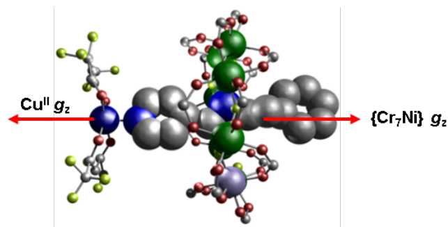
Figure 1. Crystal structure of 2 , the red arrows show the unique z axis for the \text{Cu}^{\text{II}} and \{\text{Cr}_7\text{Ni}\} . For 2 they are parallel with one another. Atom colours: blue (N), red (O), grey (C), green (Cr), lilac (Ni), navy (Cu), yellow (F). ^i\text{Bu} (pivalate) groups and hydrogens omitted for clarity
