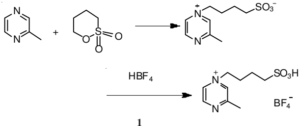
Scheme-I: Synthesis of [4-sulfbmpyrazine][BF 4 ]
