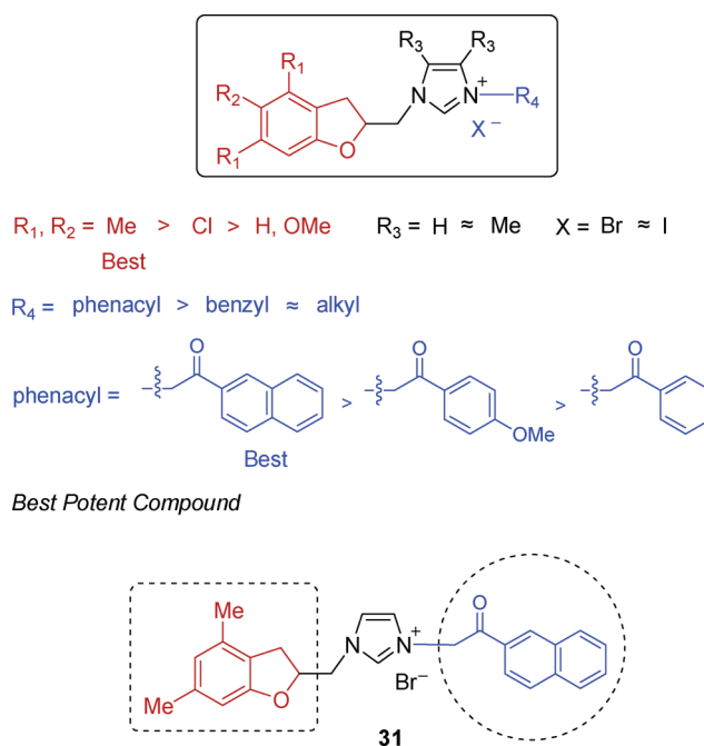
Scheme 3 Structure–activity relationship of hybrid compounds.
